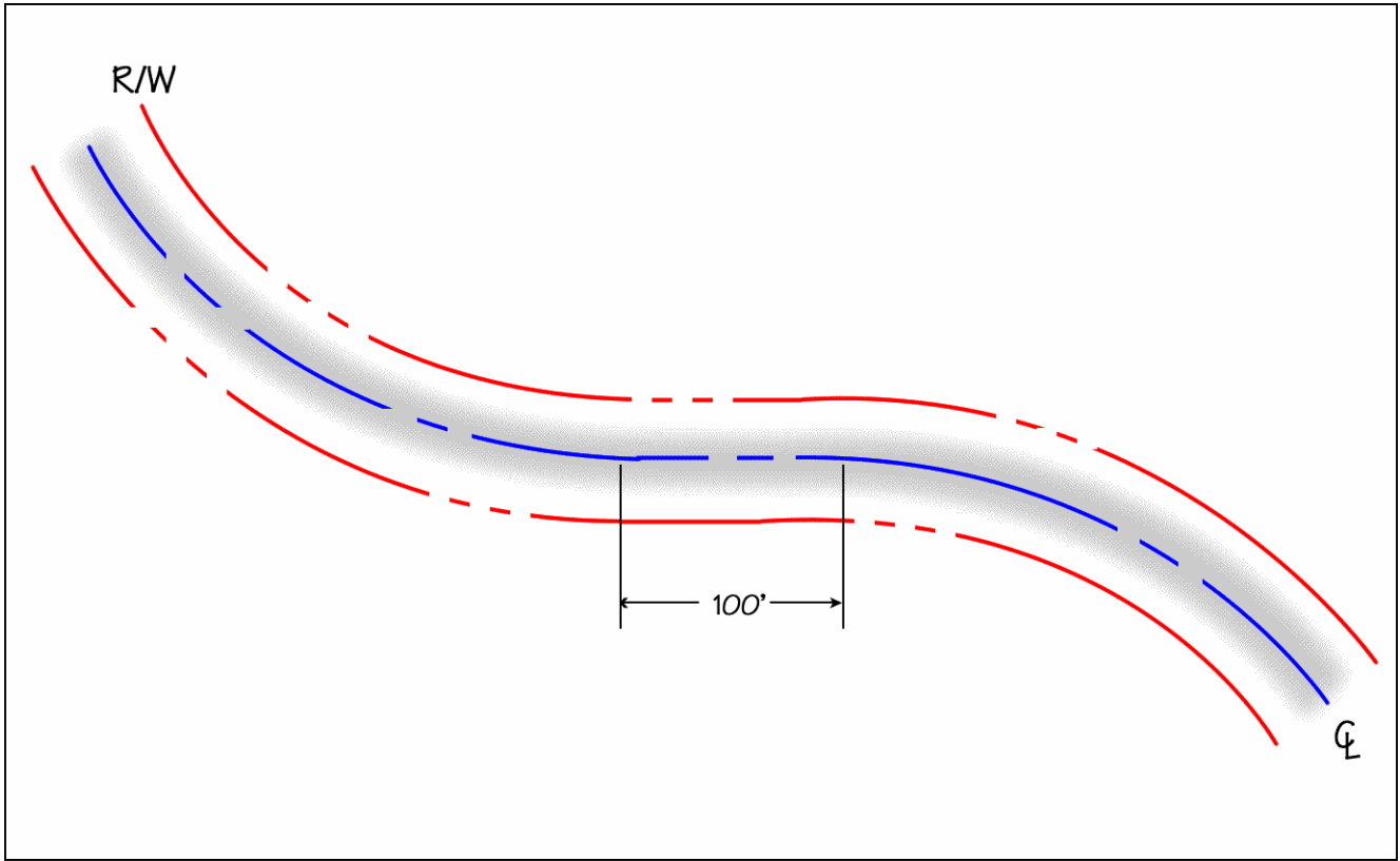
REVERSE CURVES - MINIMUM TANGENT
