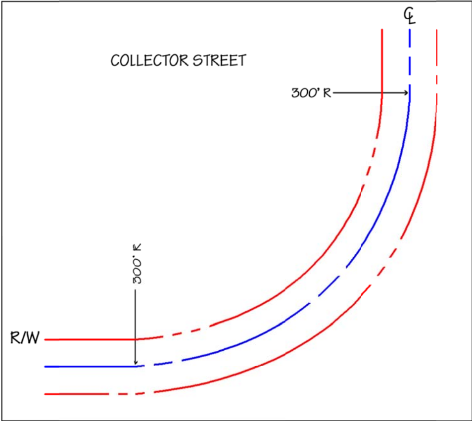
MINIMUM CURVE RADII
